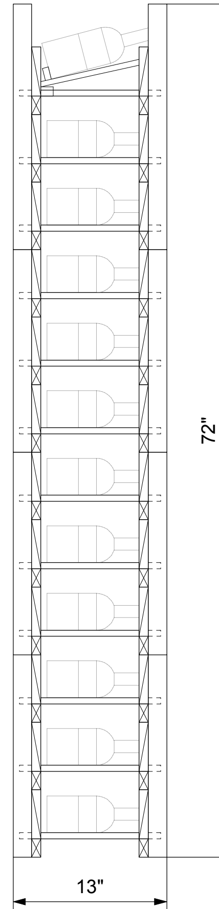
SIDE ELEVATION
